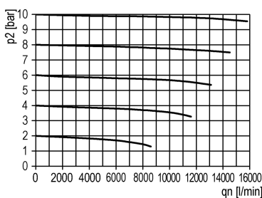
flow characteristic
